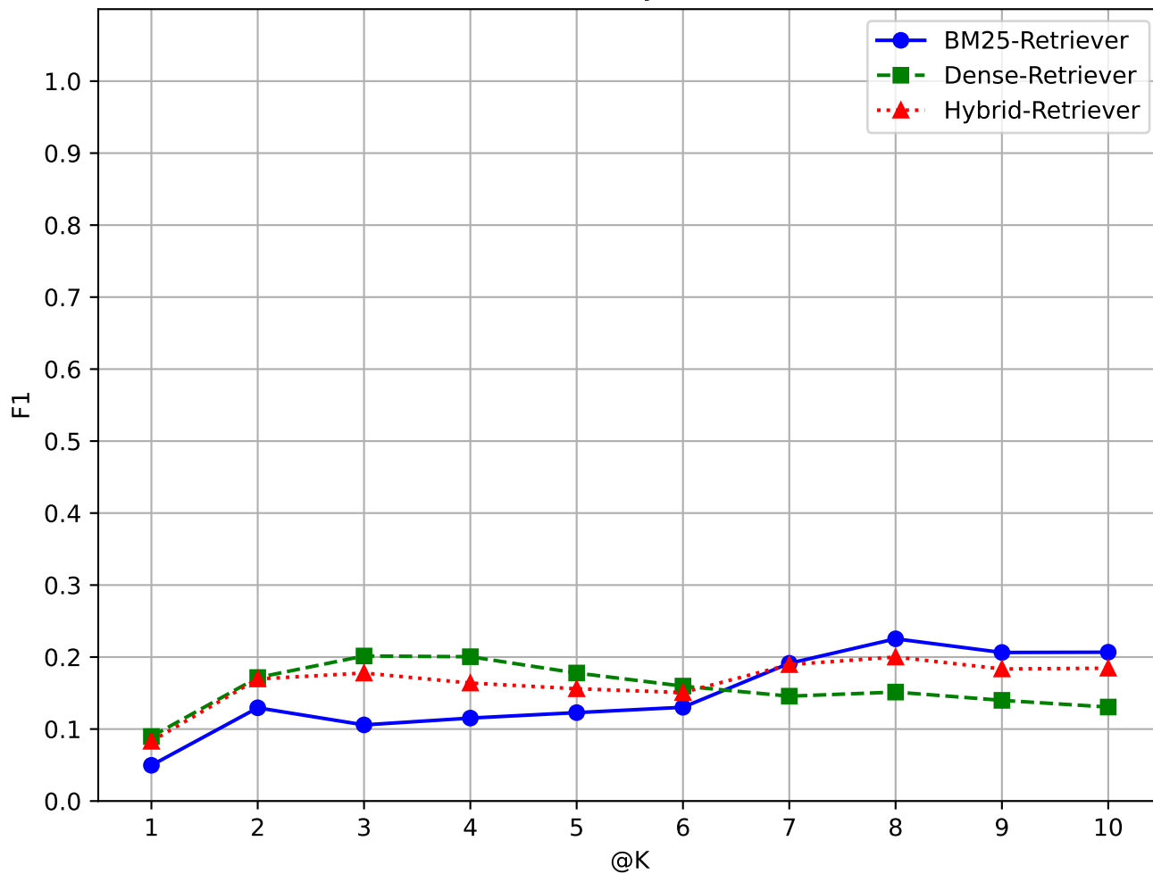
Query 6
